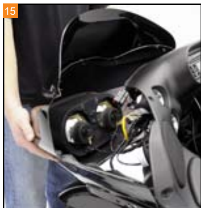
15 Remove the outer fairing.
