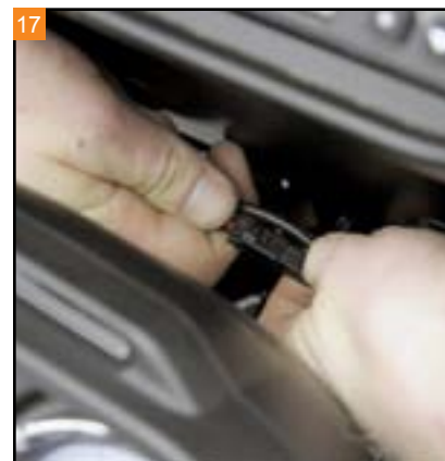
17 Plug the grip power harness into the left-grip wiring.
