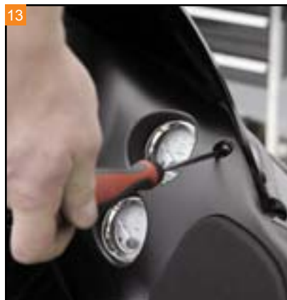
13 Remove the fairing mounting bolts.
