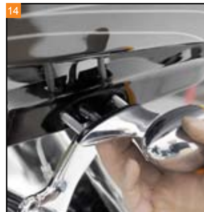
14 Remove the turn signal mounting brackets.
