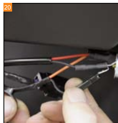
20 Plug the lighter wiring harness into the piggy-back spade connectors.
