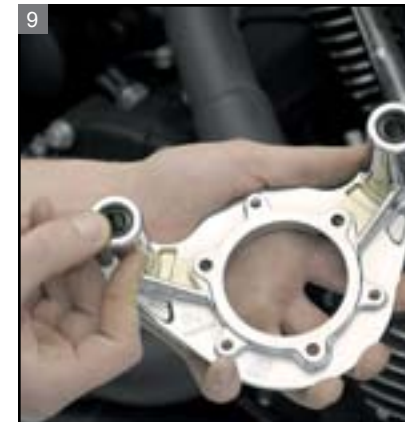
9 Install the sealing O-rings onto the new back plate.
