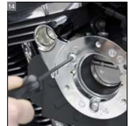
14 Install the three back plate-to-throttle body bolts.
