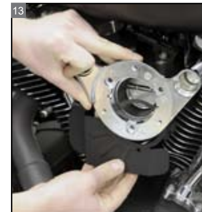
13 Slide the throttle body cover in between the back plate and throttle body.
